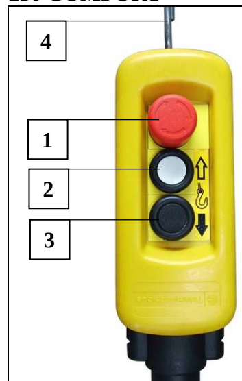
Fig. 8 Handbesturing (1-traps)
