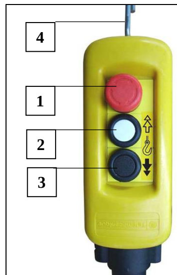
Fig. 9 Handbesturing (2-traps)
